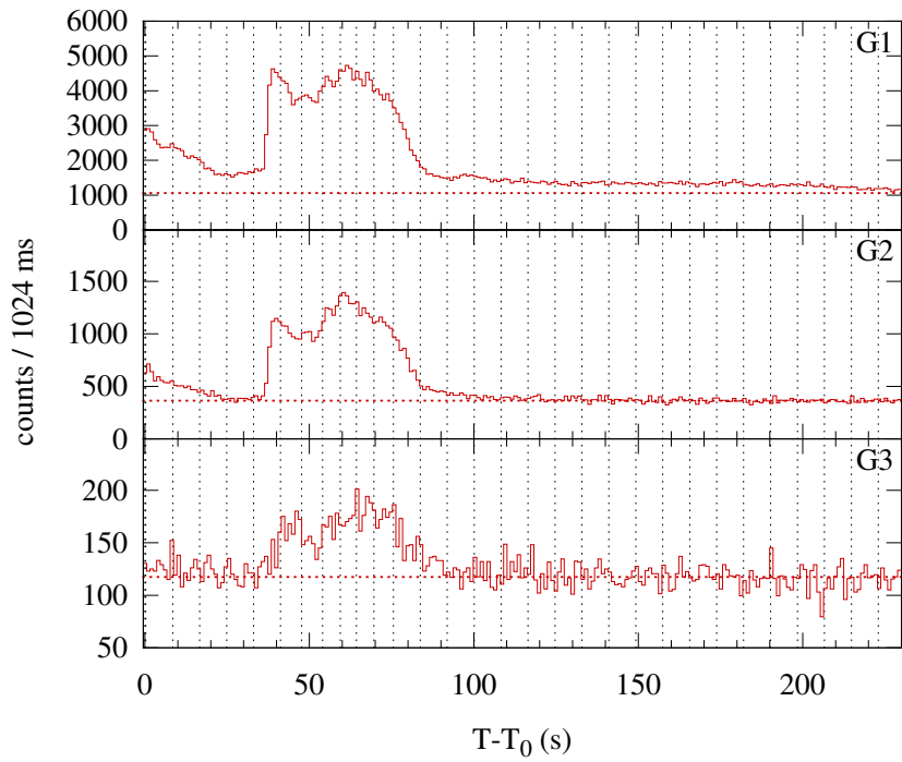
Konus-WIND S2 SOL2002-09-20T09:25 (M1.8) T 0 = 33957.677 s UT (09:25:57.677)
