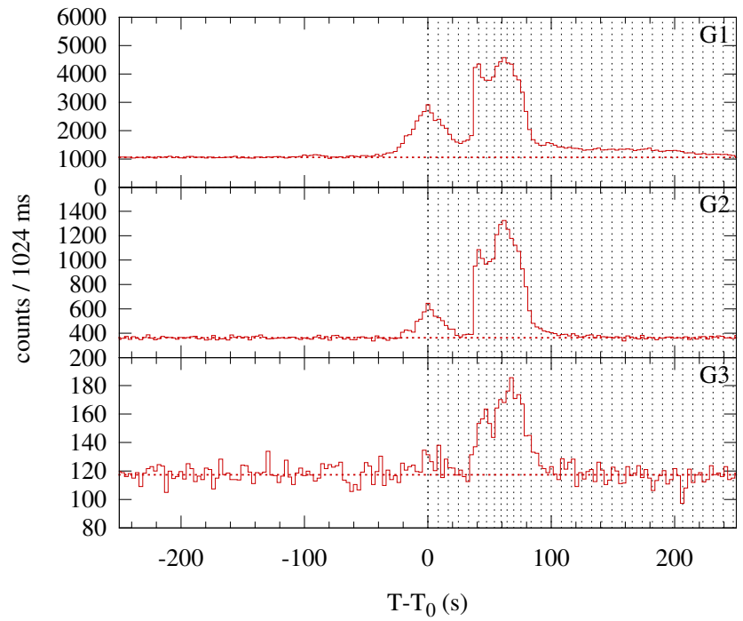
Konus-WIND S2 SOL2002-09-20T09:25 (M1.8) T 0 = 33957.677 s UT (09:25:57.677)
