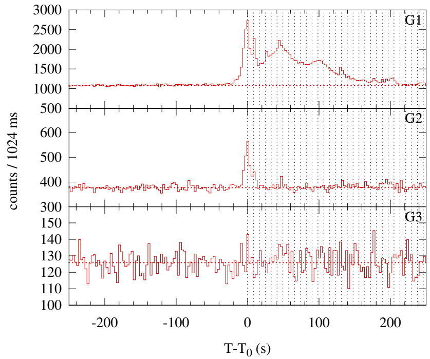
Konus-WIND S2 SOL2002-10-06T04:49 (M2.4) T_0 = 17390.8 s UT (04:49:50.8)
