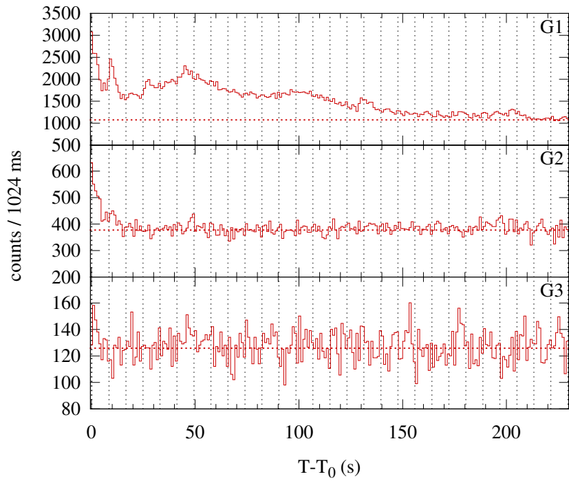
Konus-WIND S2 SOL2002-10-06T04:49 (M2.4) T_0 = 17390.8 s UT (04:49:50.8)
