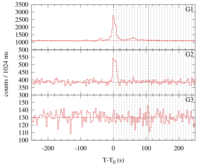
Konus-WIND S2 SOL2002-10-16T03:13 (C7.1) T_0 = 11616.288 s UT (03:13:36.288)
