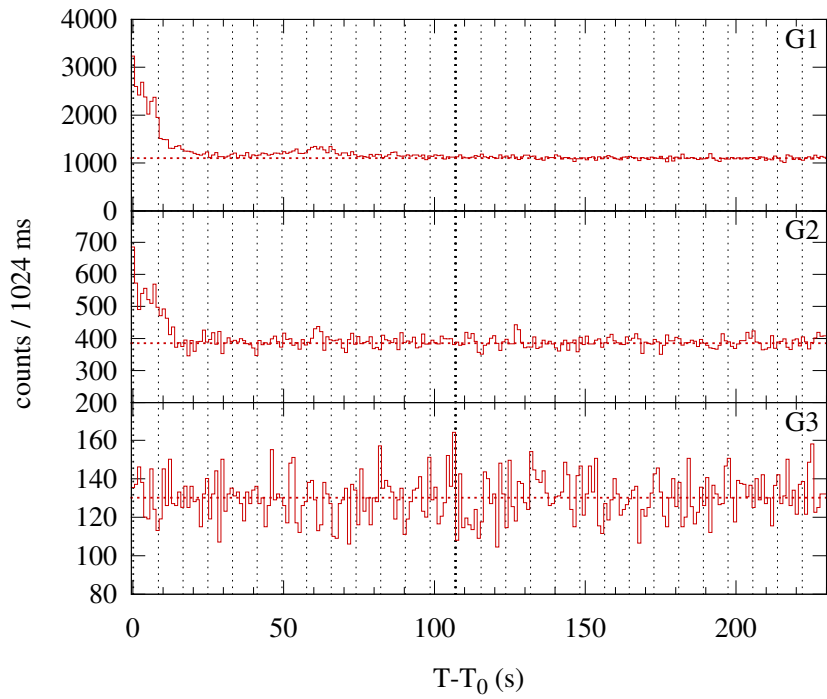
Konus-WIND S2 SOL2002-10-16T03:13 (C7.1) T_0 = 11616.288 s UT (03:13:36.288)
