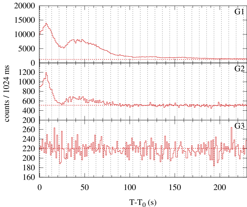
Konus-WIND S2 SOL2002-11-11T07:29 (M2.9) T_0 = 26988.763 s UT (07:29:48.763)
