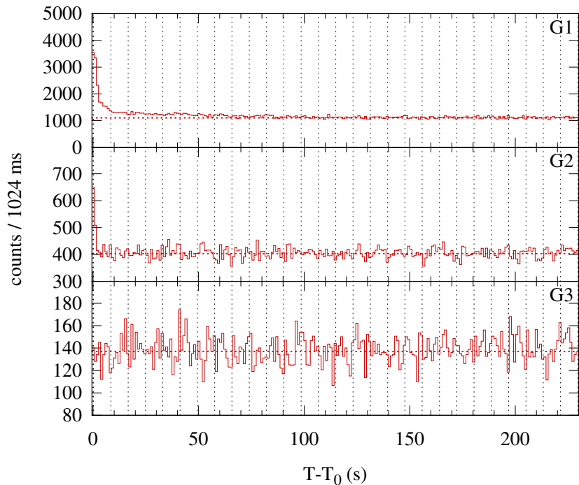
Konus-WIND S2 SOL2002-11-12T18:16 (C9.9) T 0 = 65763.743 s UT (18:16:03.743)
