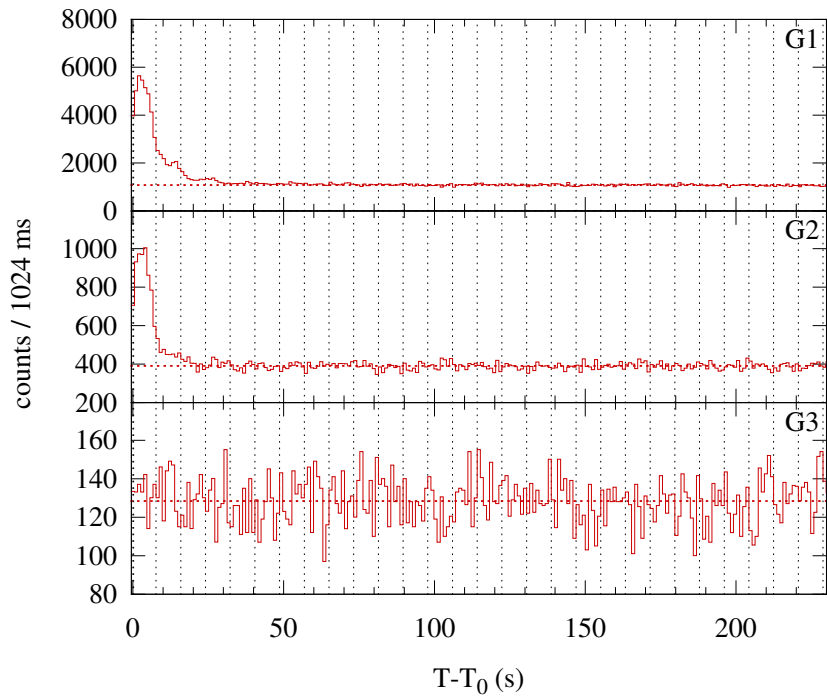
Konus-WIND S2 SOL2002-11-14T11:09 (C5.5) T_0 = 40172.456 s UT (11:09:32.456)
