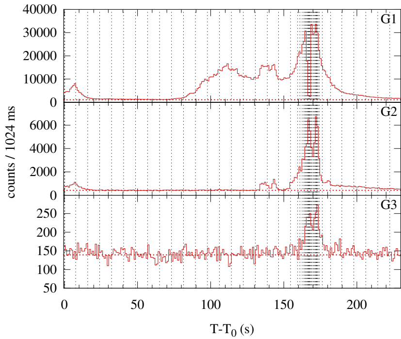
Konus-WIND S2 SOL2002-12-20T13:15 (M6.8) T_0 = 47744.638 s UT (13:15:44.638)
