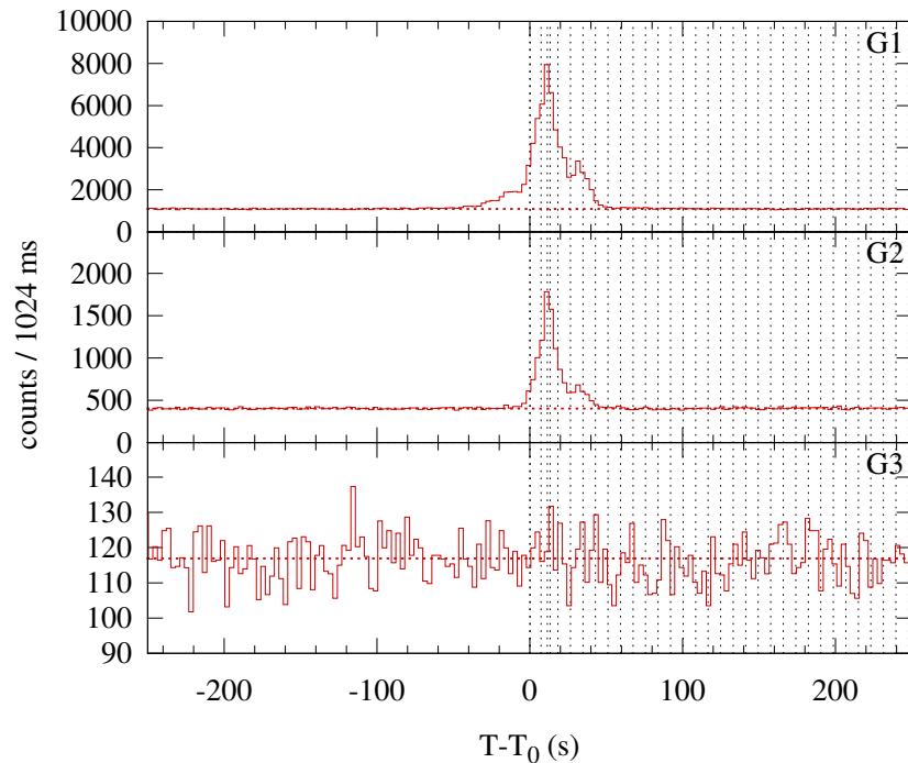
Konus-WIND S2 SOL2003-02-21T19:48 (C4.3) T_0 = 71316.554 s UT (19:48:36.554)
