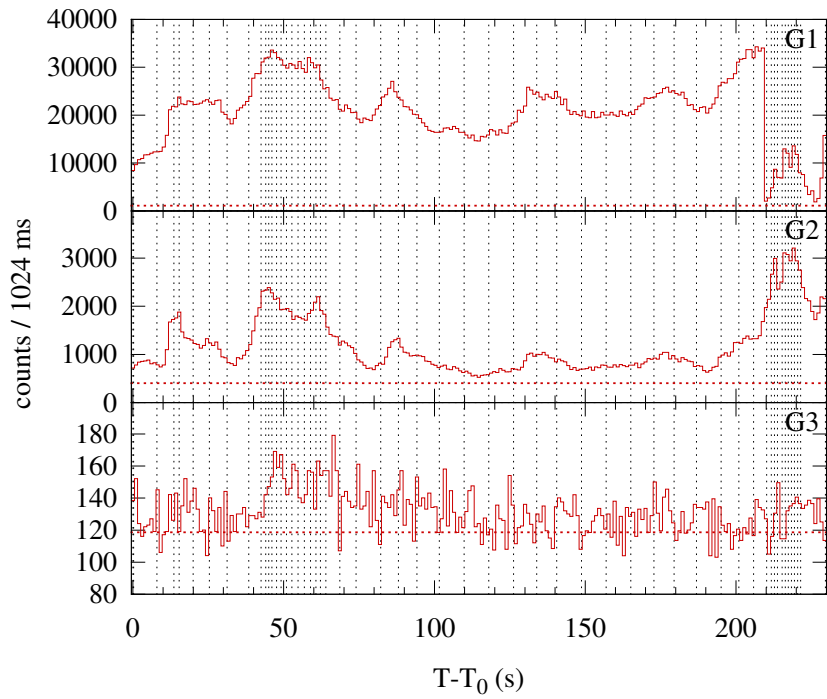
Konus-WIND S2 SOL2003-03-17T18:57 (X1.5) T_0 = 68231.621 s UT (18:57:11.621)
