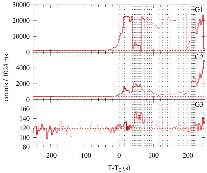
Konus-WIND S2 SOL2003-03-17T18:57 (X1.5) T_0 = 68231.621 s UT (18:57:11.621)
