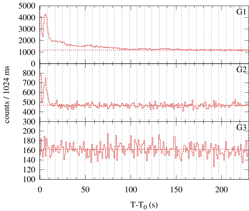
Konus-WIND S2 SOL2003-03-19T13:31 (M1.4) T_0 = 48675.293 s UT (13:31:15.293)
