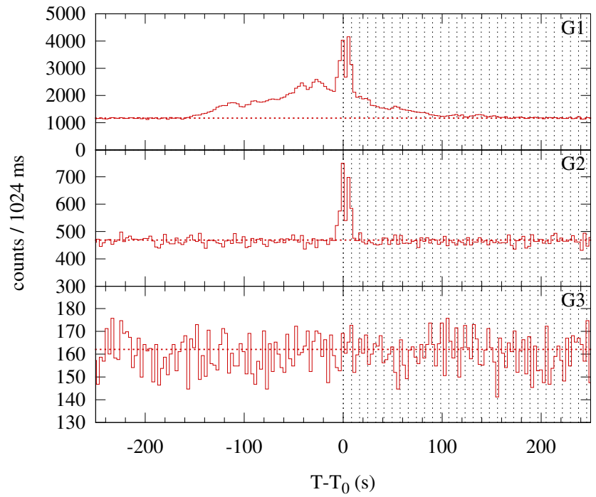
Konus-WIND S2 SOL2003-03-19T13:31 (M1.4) T_0 = 48675.293 s UT (13:31:15.293)
