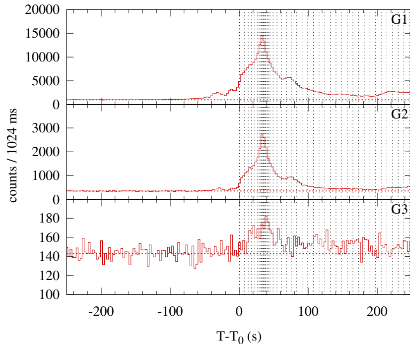
Konus-WIND S1 SOL2003-04-23T01:01 (M5.1) T 0 = 3681.10 s UT (01:01:21.10)
