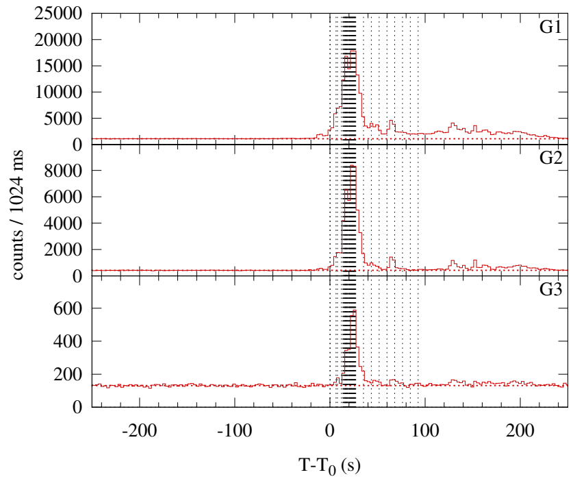
Konus-WIND S2 SOL2003-04-26T00:55 (M2.1) T_0 = 3301.0 s UT (00:55:01.0)
