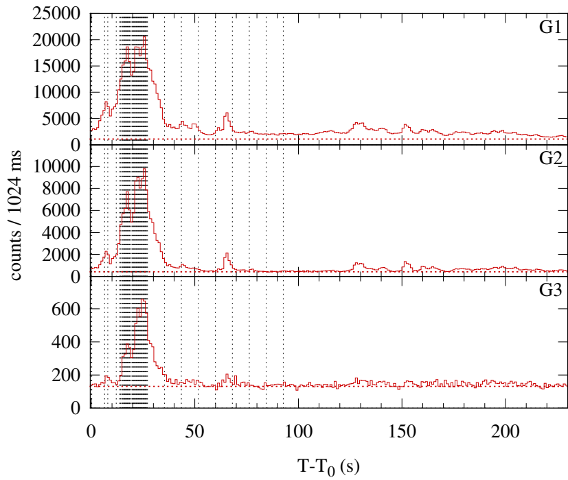
Konus-WIND S2 SOL2003-04-26T00:55 (M2.1) T_0 = 3301.0 s UT (00:55:01.0)
