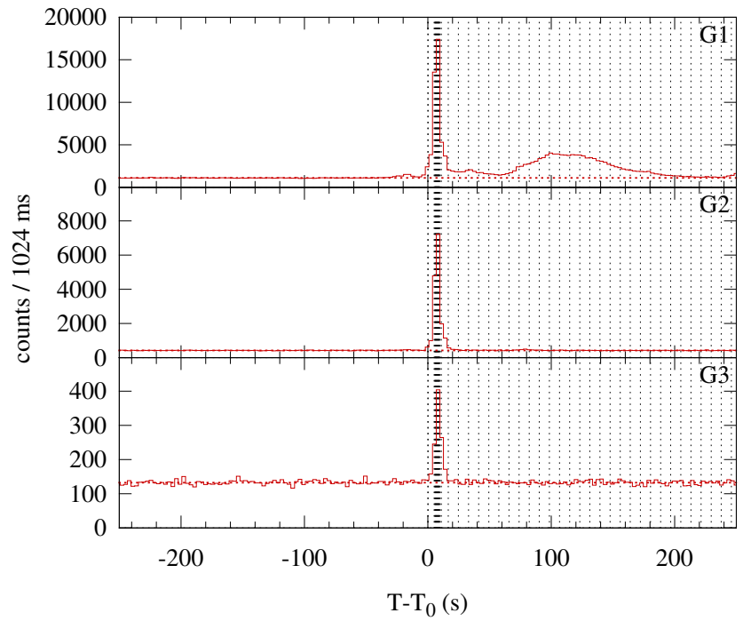
Konus-WIND S2 SOL2003-04-26T03:03 (M2.1) T_0 = 11005.460 s UT (03:03:25.460)
