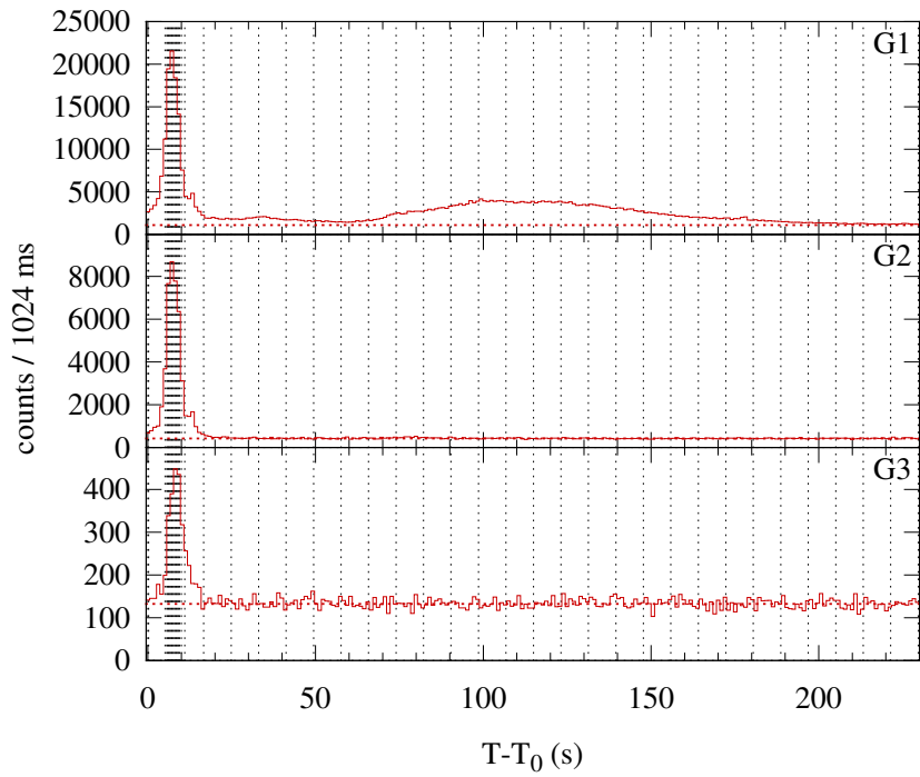
Konus-WIND S2 SOL2003-04-26T03:03 (M2.1) T_0 = 11005.460 s UT (03:03:25.460)
