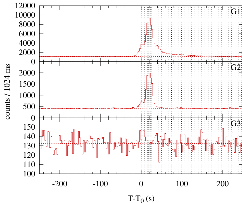
Konus-WIND S2 SOL2003-04-27T15:30 (M1.7) T_0 = 55815.712 s UT (15:30:15.712)
