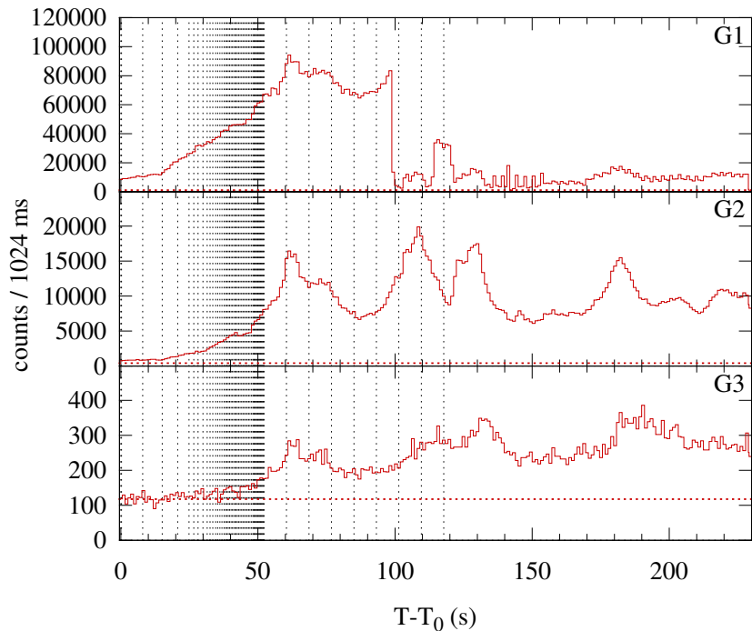
Konus-WIND S2 SOL2003-05-28T00:20 (X3.6) T_0 = 1254.185 s UT (00:20:54.185)
