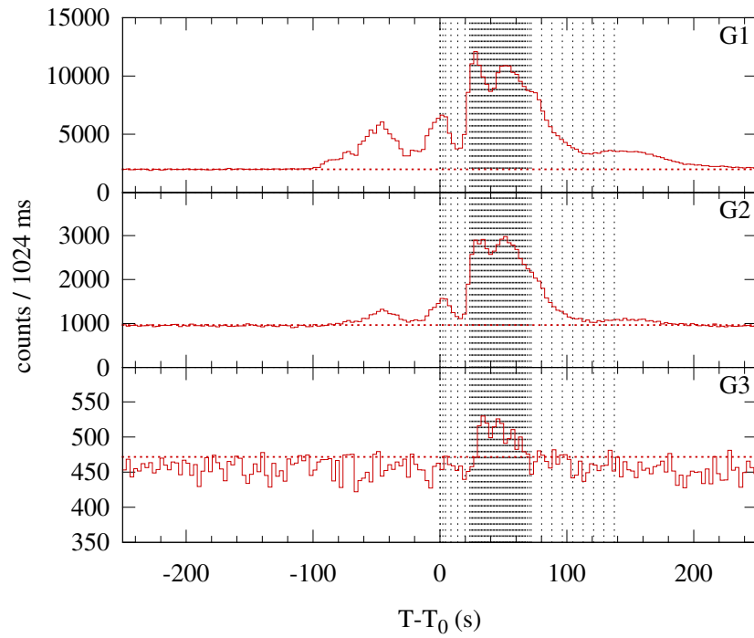
Konus-WIND S2 SOL2003-05-29T19:32 (M2.8) T_0 = 70379.1 s UT (19:32:59.1)
