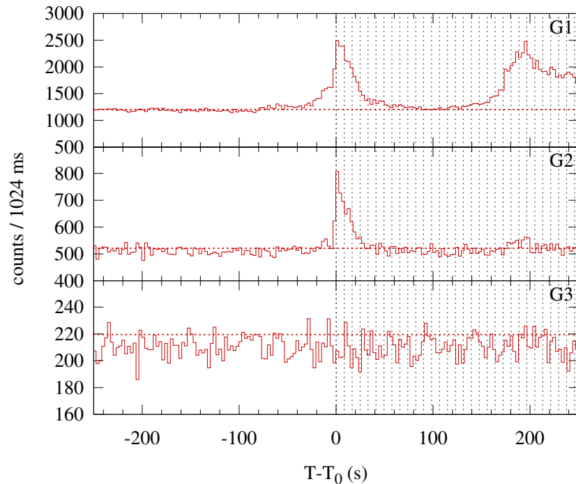
Konus-WIND S2 SOL2003-06-01T07:04 (M1.0) T_0 = 25467.331 s UT (07:04:27.331)
