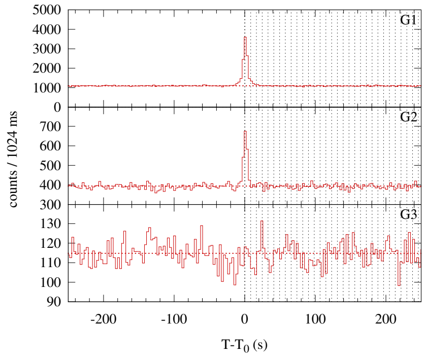
Konus-WIND S2 SOL2003-06-07T09:41 (C2.3) T 0 = 34909.308 s UT (09:41:49.308)
