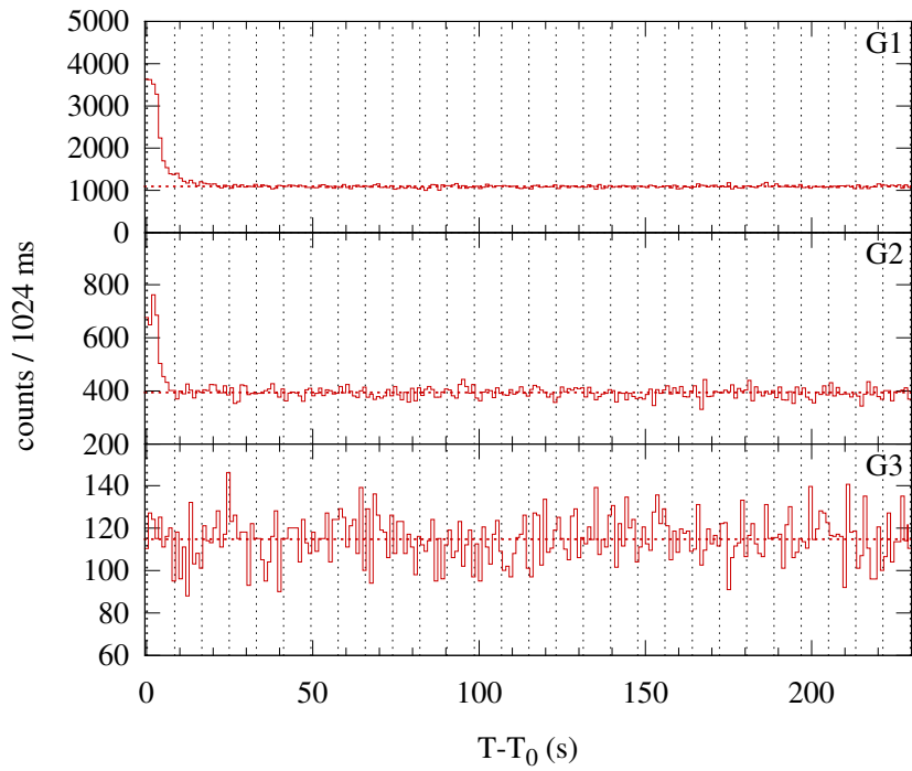
Konus-WIND S2 SOL2003-06-07T09:41 (C2.3) T 0 = 34909.308 s UT (09:41:49.308)
