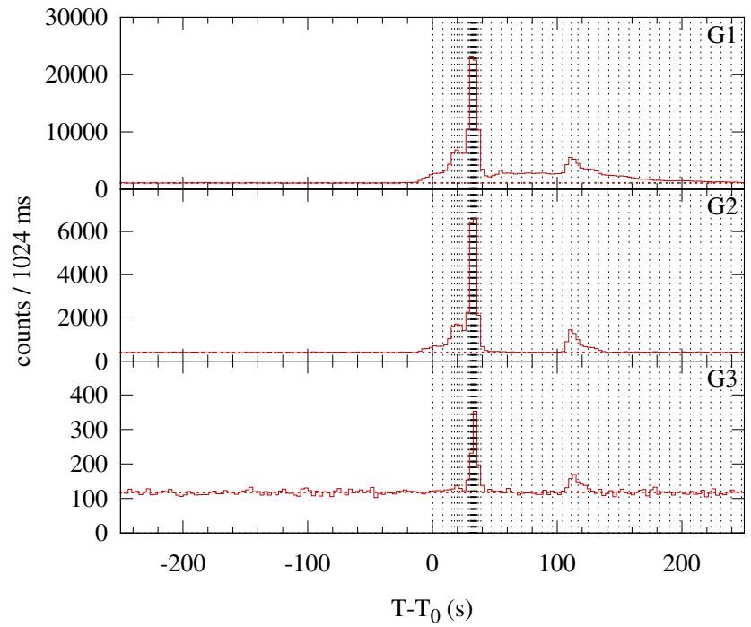
Konus-WIND S2 SOL2003-06-10T08:35 (M2.7) T_0 = 30926.520 s UT (08:35:26.520)
