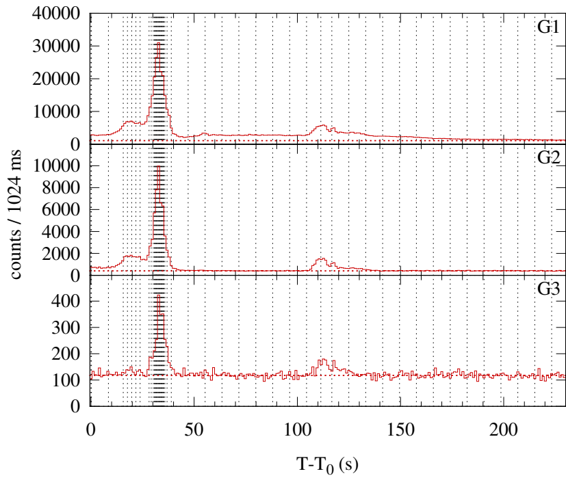
Konus-WIND S2 SOL2003-06-10T08:35 (M2.7) T_0 = 30926.520 s UT (08:35:26.520)
