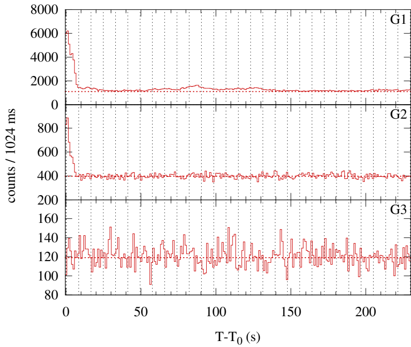
Konus-WIND S2 SOL2003-06-12T14:00 (M1.0) T 0 = 50433.166 s UT (14:00:33.166)
