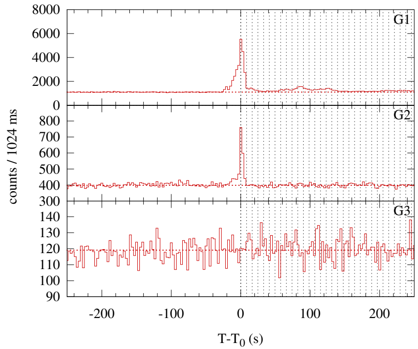
Konus-WIND S2 SOL2003-06-12T14:00 (M1.0) T 0 = 50433.166 s UT (14:00:33.166)
