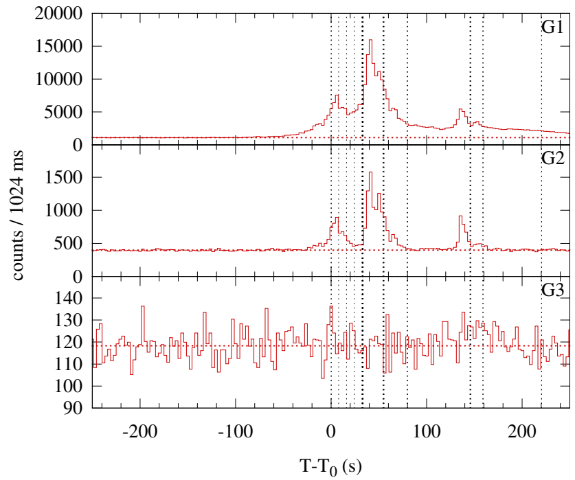
Konus-WIND S2 SOL2003-06-12T21:24 (M2.6) T_0 = 77058.709 s UT (21:24:18.709)
