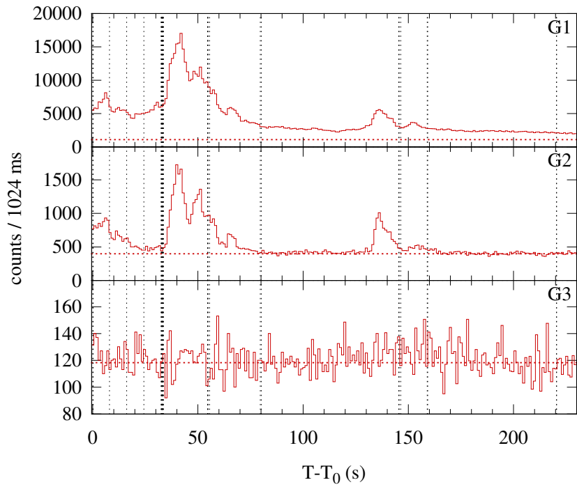
Konus-WIND S2 SOL2003-06-12T21:24 (M2.6) T_0 = 77058.709 s UT (21:24:18.709)
