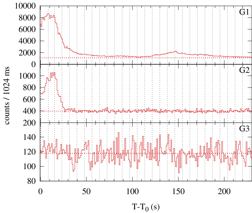
Konus-WIND S2 SOL2003-08-02T23:50 (M1.3) T_0 = 85852.481 s UT (23:50:52.481)
