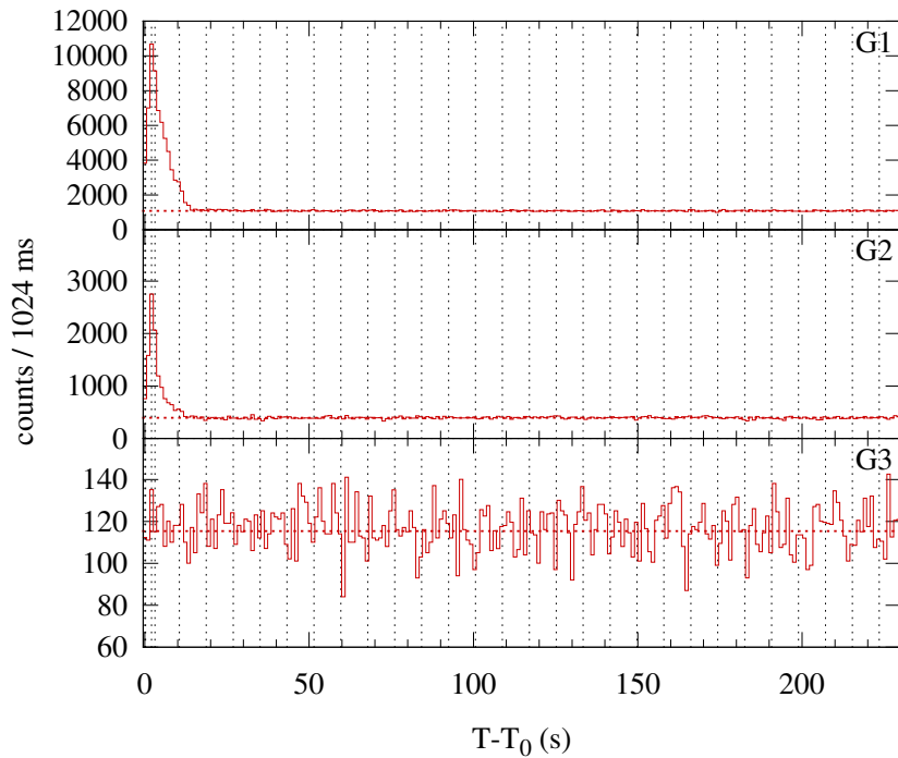
Konus-WIND S2 SOL2003-08-10T01:26 (C1.8) T 0 = 5182.265 s UT (01:26:22.265)
