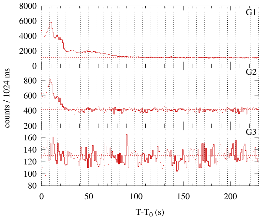
Konus-WIND S2 SOL2003-10-20T22:00 (C6.2) T 0 = 79208.410 s UT (22:00:08.410)
