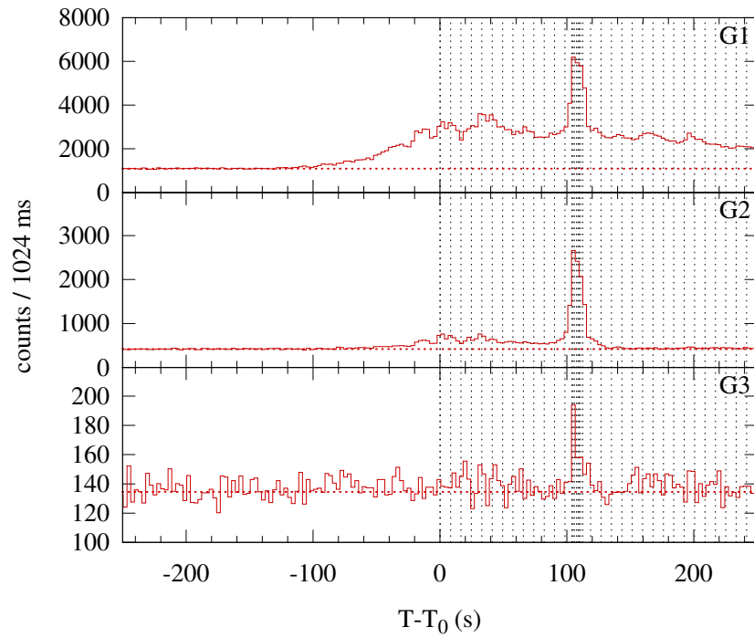
Konus-WIND S2 SOL2003-10-22T03:28 (M3.7) T_0 = 12510.680 s UT (03:28:30.680)
