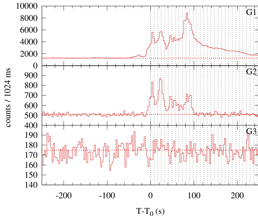
Konus-WIND S2 SOL2003-10-23T02:38 (M2.4) T_0 = 9506.171 s UT (02:38:26.171)
