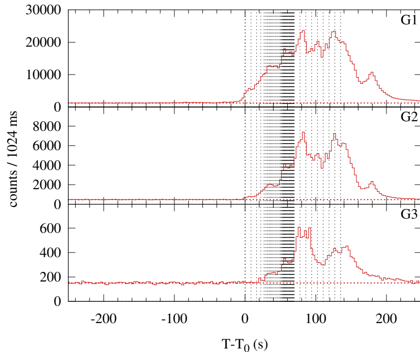
Konus-WIND S2 SOL2003-10-24T05:06 (M4.2) T_0 = 18404.755 s UT (05:06:44.755)
