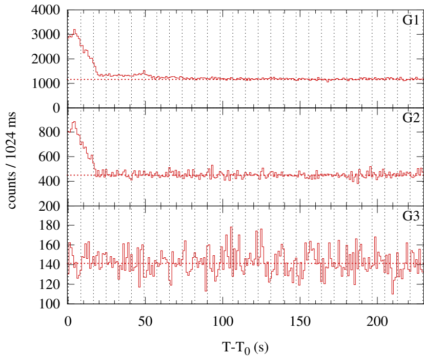
Konus-WIND S2 SOL2003-10-24T20:23 (C5.3) T 0 = 73408.376 s UT (20:23:28.376)
