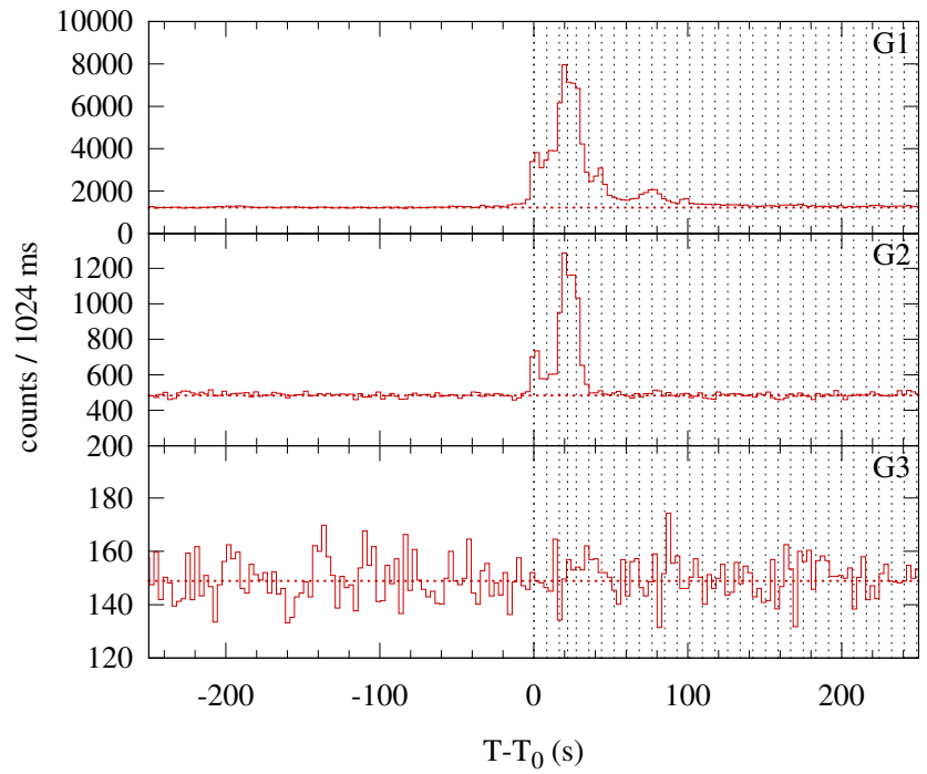
Konus-WIND S2 SOL2003-10-24T21:38 (M1.0) T 0 = 77906.789 s UT (21:38:26.789)
