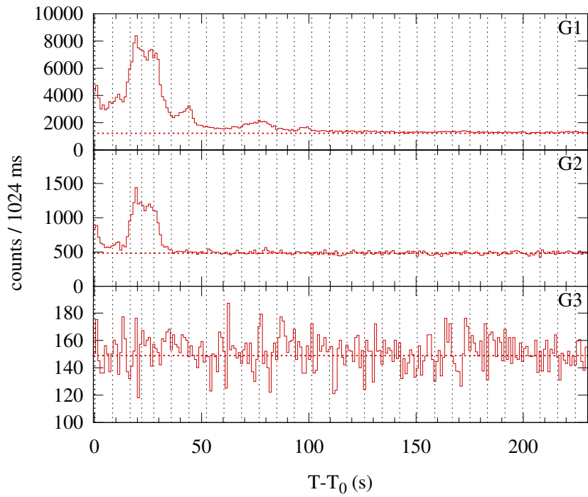
Konus-WIND S2 SOL2003-10-24T21:38 (M1.0) T 0 = 77906.789 s UT (21:38:26.789)
