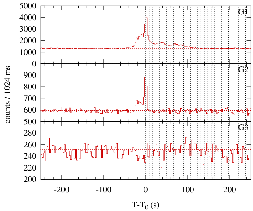
Konus-WIND S2 SOL2003-10-28T05:10 (C7.7) T 0 = 18613.772 s UT (05:10:13.772)
