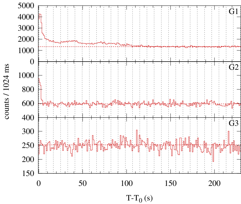
Konus-WIND S2 SOL2003-10-28T05:10 (C7.7) T 0 = 18613.772 s UT (05:10:13.772)
