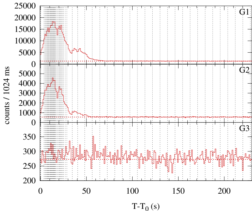
Konus-WIND S2 SOL2003-11-20T07:26 (C3.8) T_0 = 26797.812 s UT (07:26:37.812)
