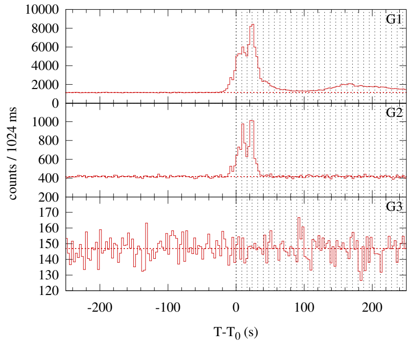
Konus-WIND S2 SOL2003-12-06T15:40 (M2.0) T 0 = 56458.996 s UT (15:40:58.996)
