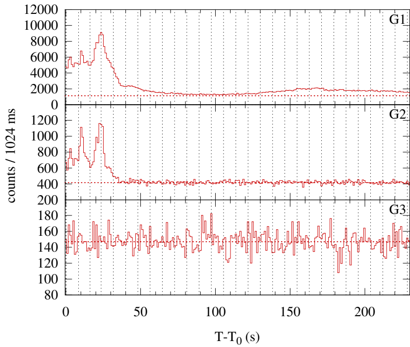
Konus-WIND S2 SOL2003-12-06T15:40 (M2.0) T 0 = 56458.996 s UT (15:40:58.996)
