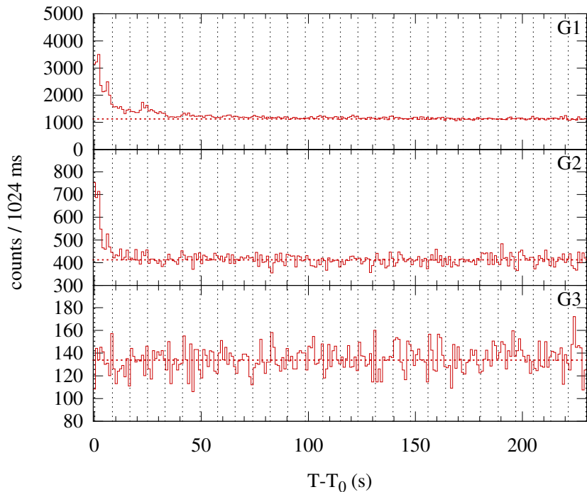
Konus-WIND S2 SOL2003-12-19T16:44 (C5.4) T 0 = 60299.30 s UT (16:44:59.30)
