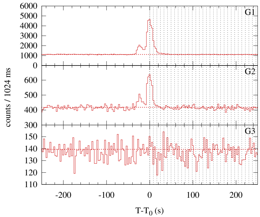
Konus-WIND S2 SOL2004-01-01T06:52 (C8.0) T 0 = 24765.142 s UT (06:52:45.142)
