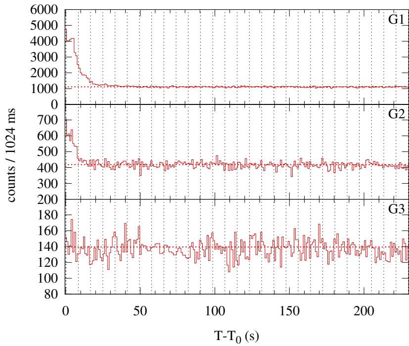
Konus-WIND S2 SOL2004-01-01T06:52 (C8.0) T 0 = 24765.142 s UT (06:52:45.142)
