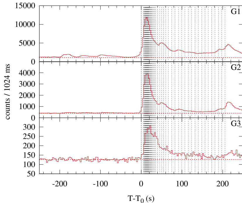
Konus-WIND S2 SOL2004-01-06T06:22 (M5.8) T_0 = 22946.499 s UT (06:22:26.499)
