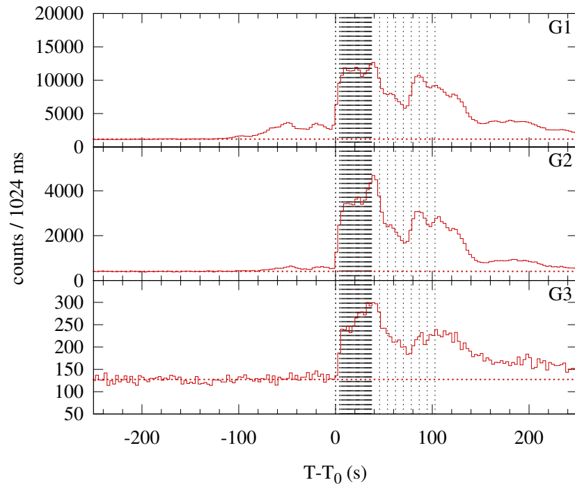
Konus-WIND S2 SOL2004-01-07T03:56 (M4.5) T_0 = 14177.386 s UT (03:56:17.386)
