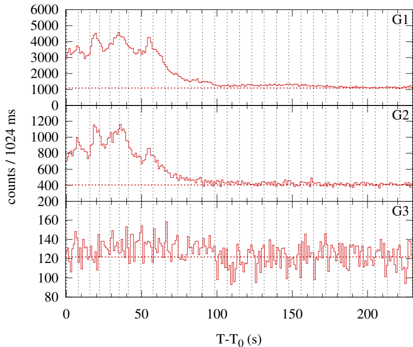
Konus-WIND S2 SOL2004-02-04T11:15 (C9.9) T 0 = 40516.972 s UT (11:15:16.972)
