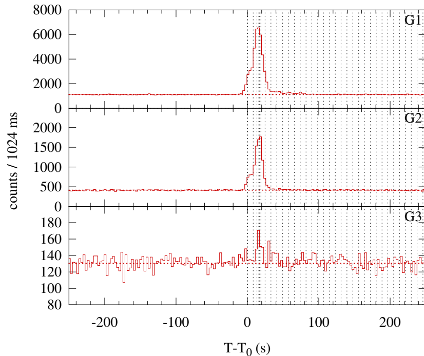
Konus-WIND S2 SOL2004-03-30T09:44 (C5.9) T 0 = 35083.570 s UT (09:44:43.570)
