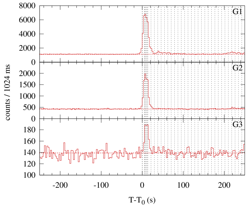
Konus-WIND S2 SOL2004-03-30T12:56 (C4.7) T 0 = 46582.182 s UT (12:56:22.182)
