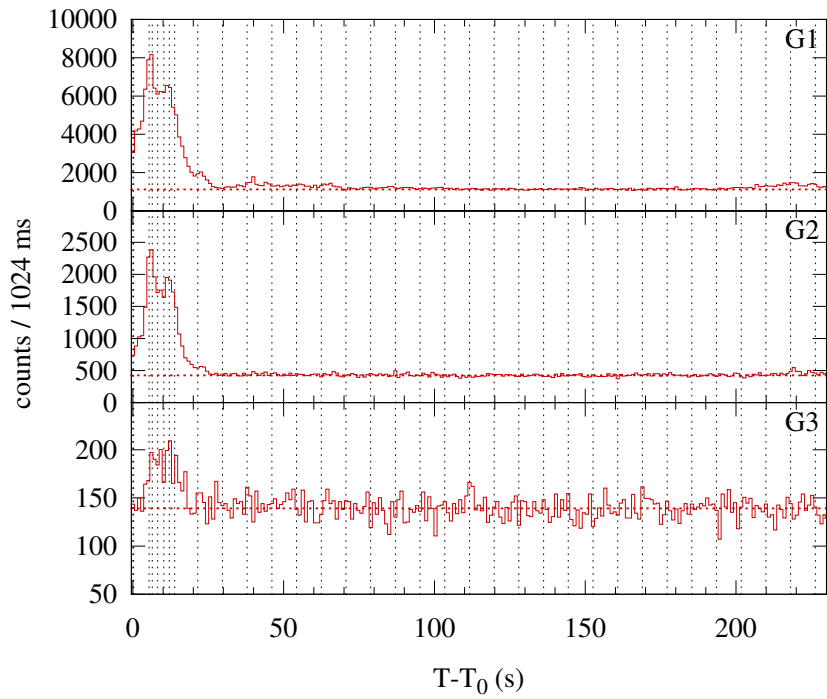
Konus-WIND S2 SOL2004-03-30T12:56 (C4.7) T 0 = 46582.182 s UT (12:56:22.182)
