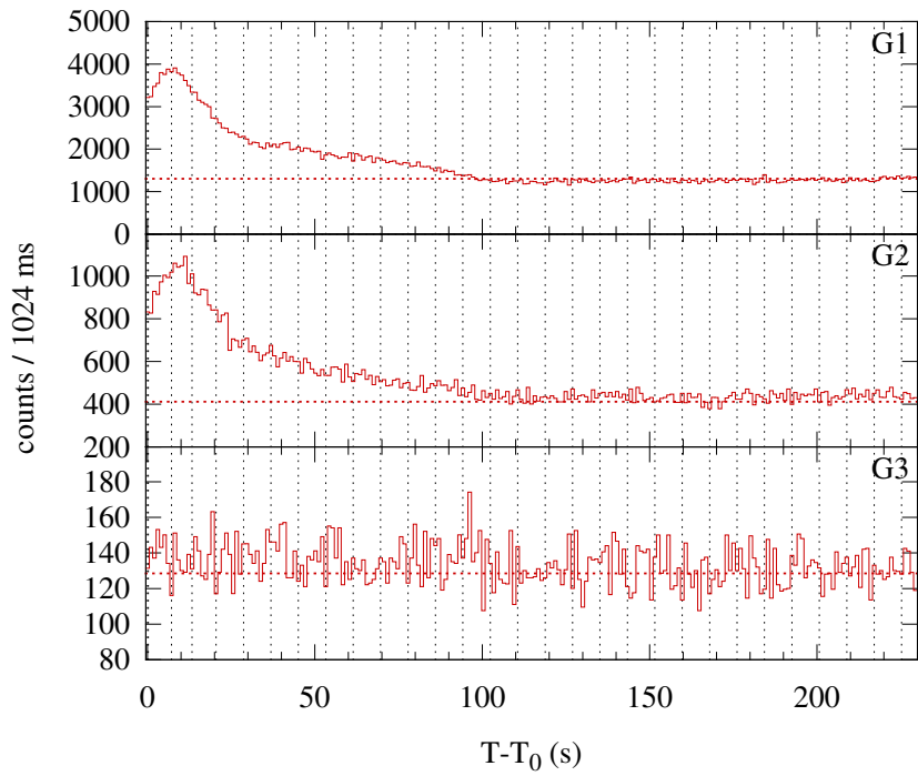
Konus-WIND S2 SOL2004-04-11T04:15 (C9.6) T_0 = 15316.2 s UT (04:15:16.2)
