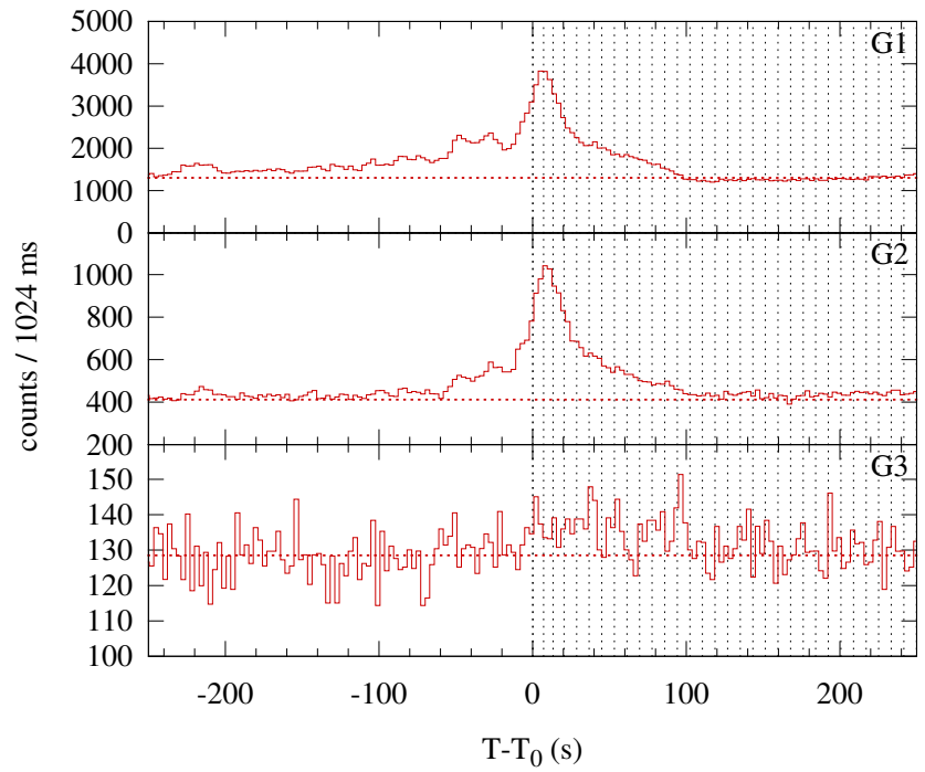
Konus-WIND S2 SOL2004-04-11T04:15 (C9.6) T_0 = 15316.2 s UT (04:15:16.2)
