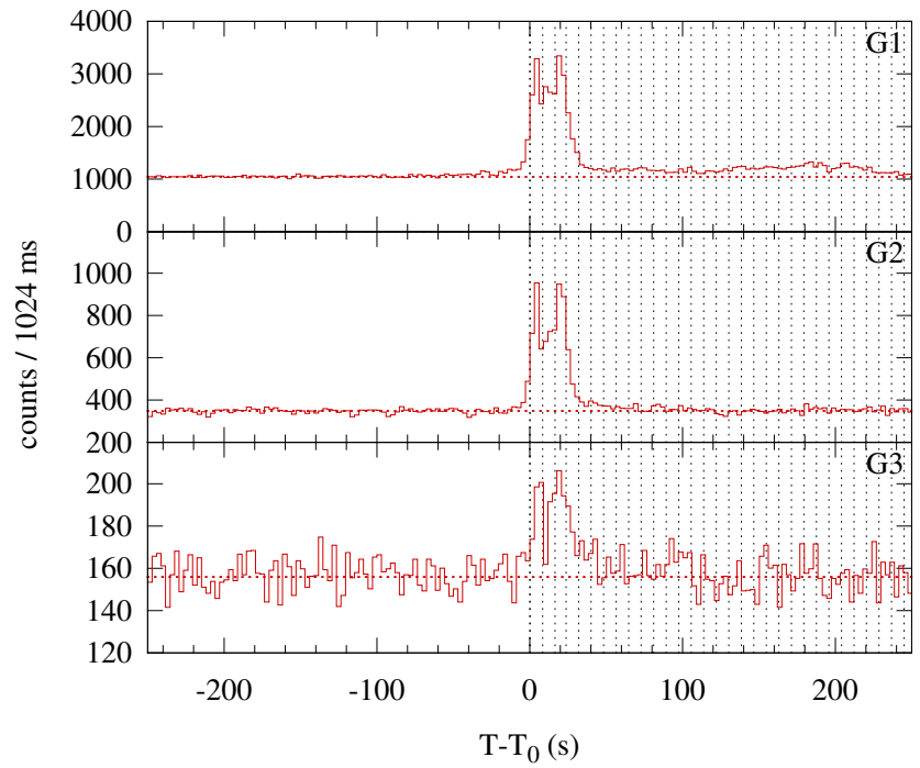
Konus-WIND S1 SOL2004-04-23T21:09 (M1.1) T 0 = 76148.854 s UT (21:09:08.854)
