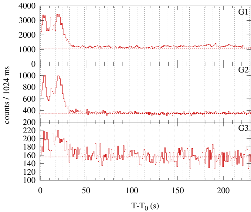
Konus-WIND S1 SOL2004-04-23T21:09 (M1.1) T 0 = 76148.854 s UT (21:09:08.854)
