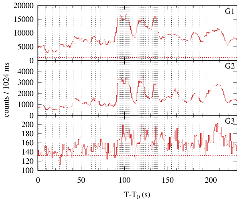
Konus-WIND S2 SOL2004-07-13T00:13 (M6.7) T_0 = 800.798 s UT (00:13:20.798)
