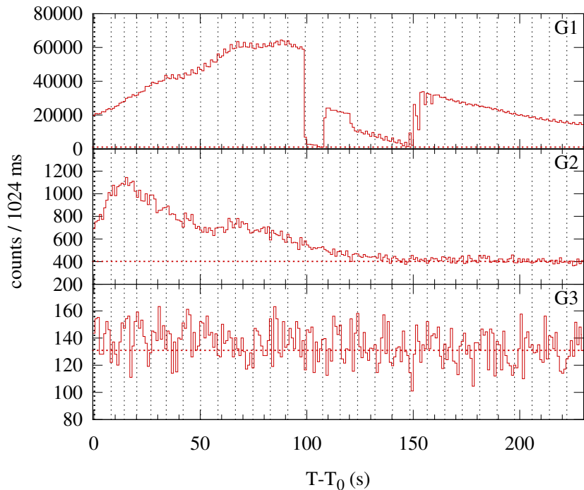
Konus-WIND S2 SOL2004-07-15T01:37 (X1.8) T_0 = 5874.923 s UT (01:37:54.923)
