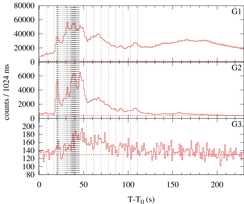
Konus-WIND S2 SOL2004-07-16T02:02 (X1.3) T 0 = 7330.530 s UT (02:02:10.530)
