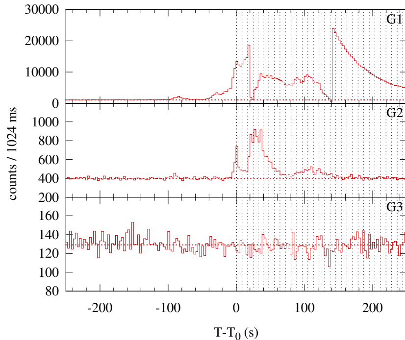
Konus-WIND S2 SOL2004-07-16T10:38 (X1.1) T 0 = 38306.393 s UT (10:38:26.393)
