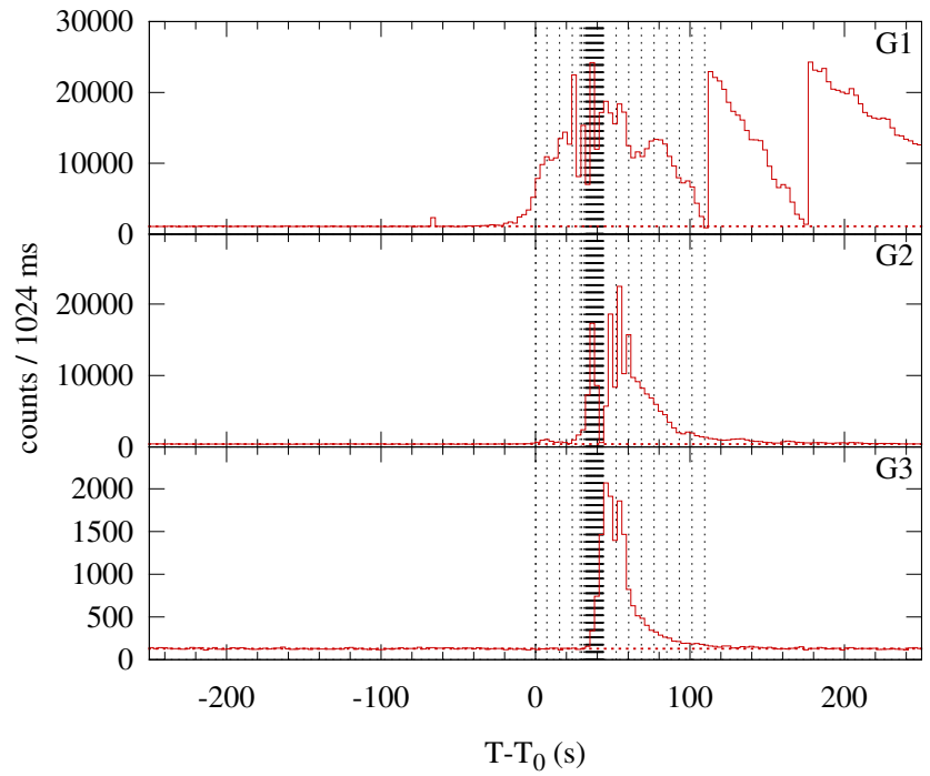
Konus-WIND S2 SOL2004-07-16T13:52 (X3.6) T_0 = 49975.853 s UT (13:52:55.853)
