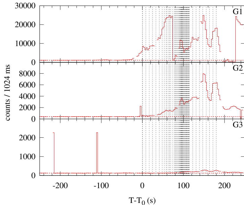
Konus-WIND S2 SOL2004-07-20T12:26 (M8.6) T_0 = 44781.490 s UT (12:26:21.490)
