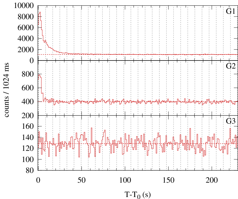
Konus-WIND S2 SOL2004-07-21T00:32 (C6.6) T 0 = 1957.215 s UT (00:32:37.215)
