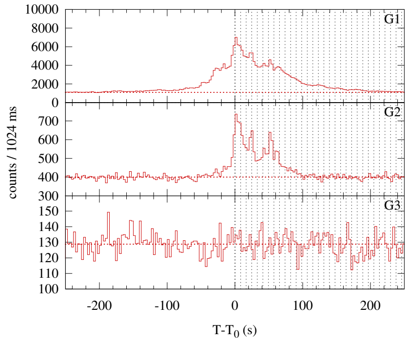
Konus-WIND S2 SOL2004-07-21T05:14 (C8.9) T_0 = 18889.431 s UT (05:14:49.431)
