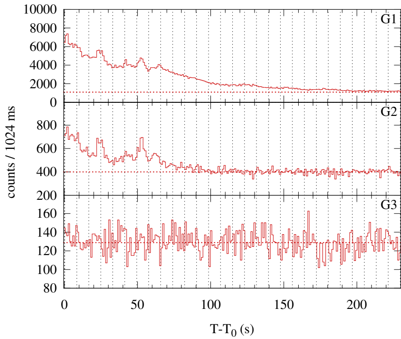
Konus-WIND S2 SOL2004-07-21T05:14 (C8.9) T_0 = 18889.431 s UT (05:14:49.431)
