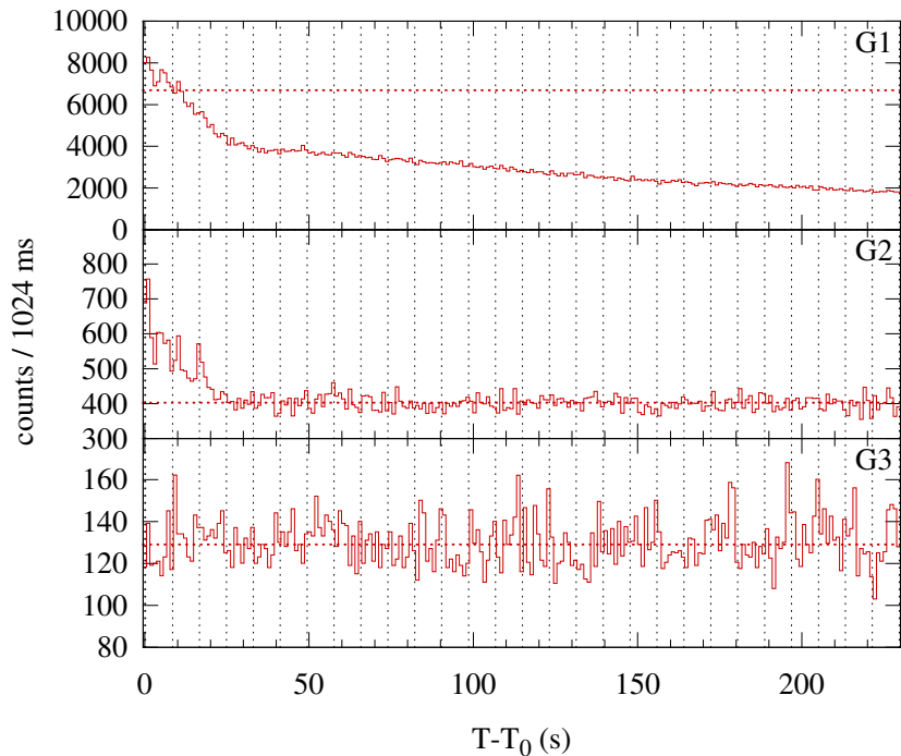
Konus-WIND S2 SOL2004-07-22T00:31 (M9.1) T 0 = 1868.868 s UT (00:31:08.868)
